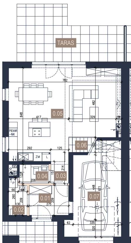
PARTER - 82,53m 2
